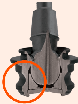
PATENTED BALL JOINT INTERNALS Limits flattening of spring disc over service life, creating a longer lasting and tighter assembly.
