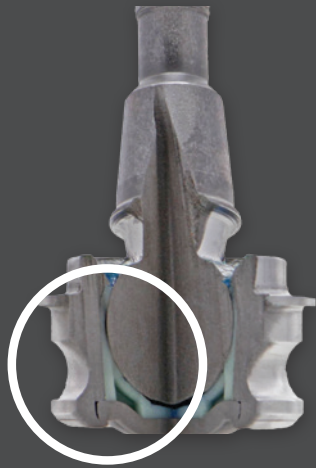
OEM BALL JOINT Polymer bearing with sealed design
